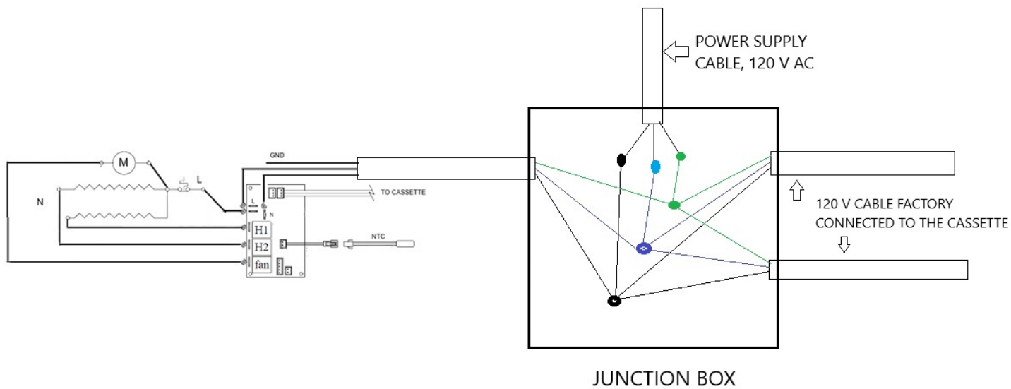
Cassette wiring diagram
