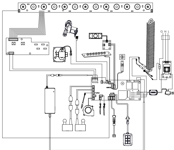
Cassette wiring diagram
